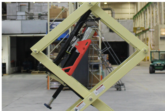
Capture shield for lift cylinder
