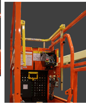
INTEGRATED MID-RAIL DECK KIT
